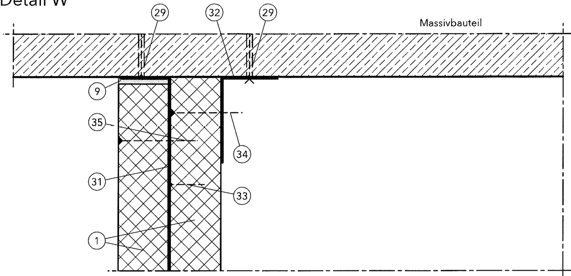
Detail W
