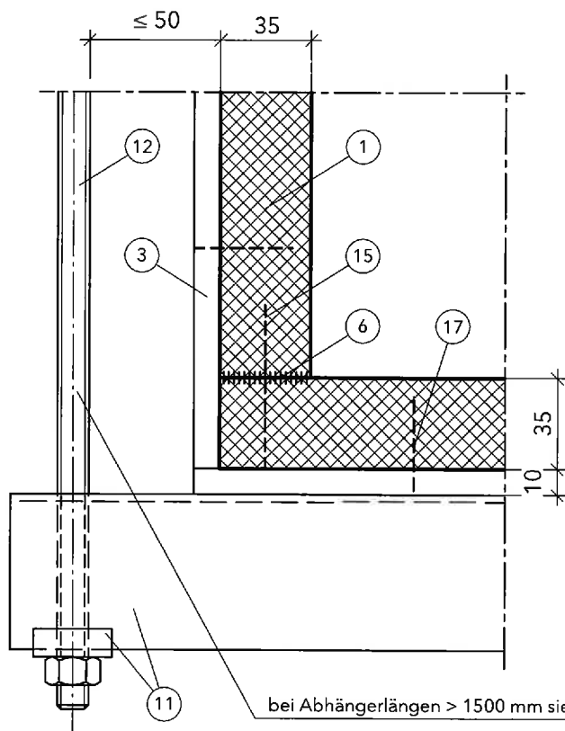
Detail B
