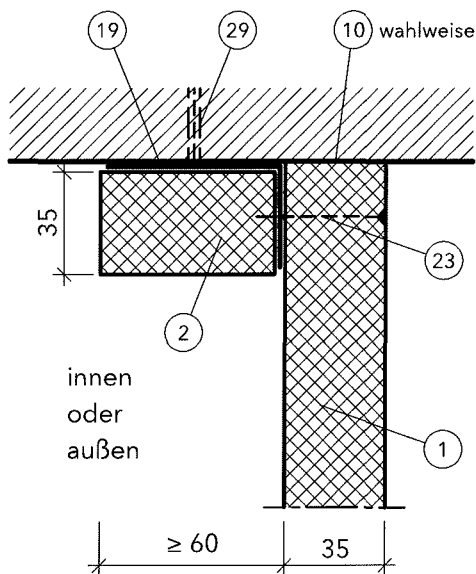
Detail G
