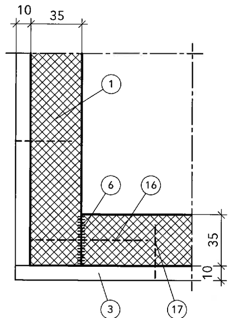
Detail B - Alternative
