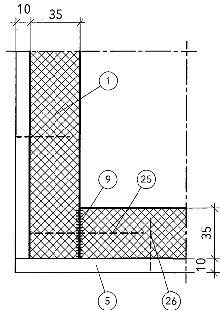
Detail B - Alternative
