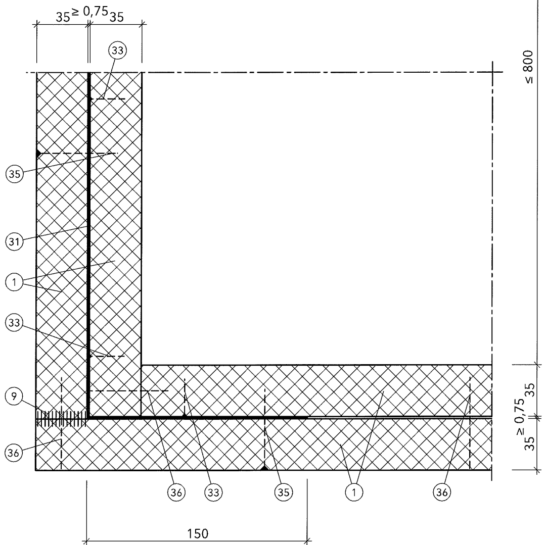
Detail X
