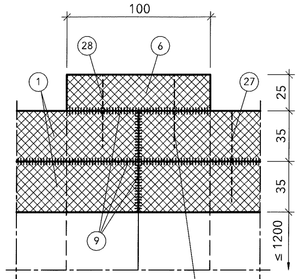
Detail P
