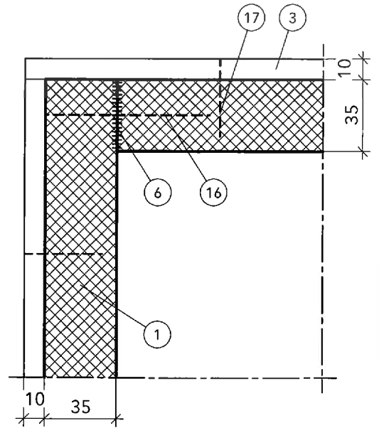
Detail A - Alternative
